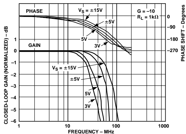
Figure 38. Closed-Loop Gain and Phase vs. Frequency, Gain = -10, R_L = 1\ \text{k}\Omega
