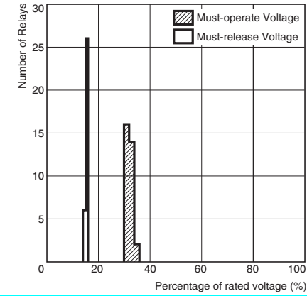
● Must-operate Voltage and Must-release Voltage Distributions (Number of Relays x Percentage of Rated Voltage)
