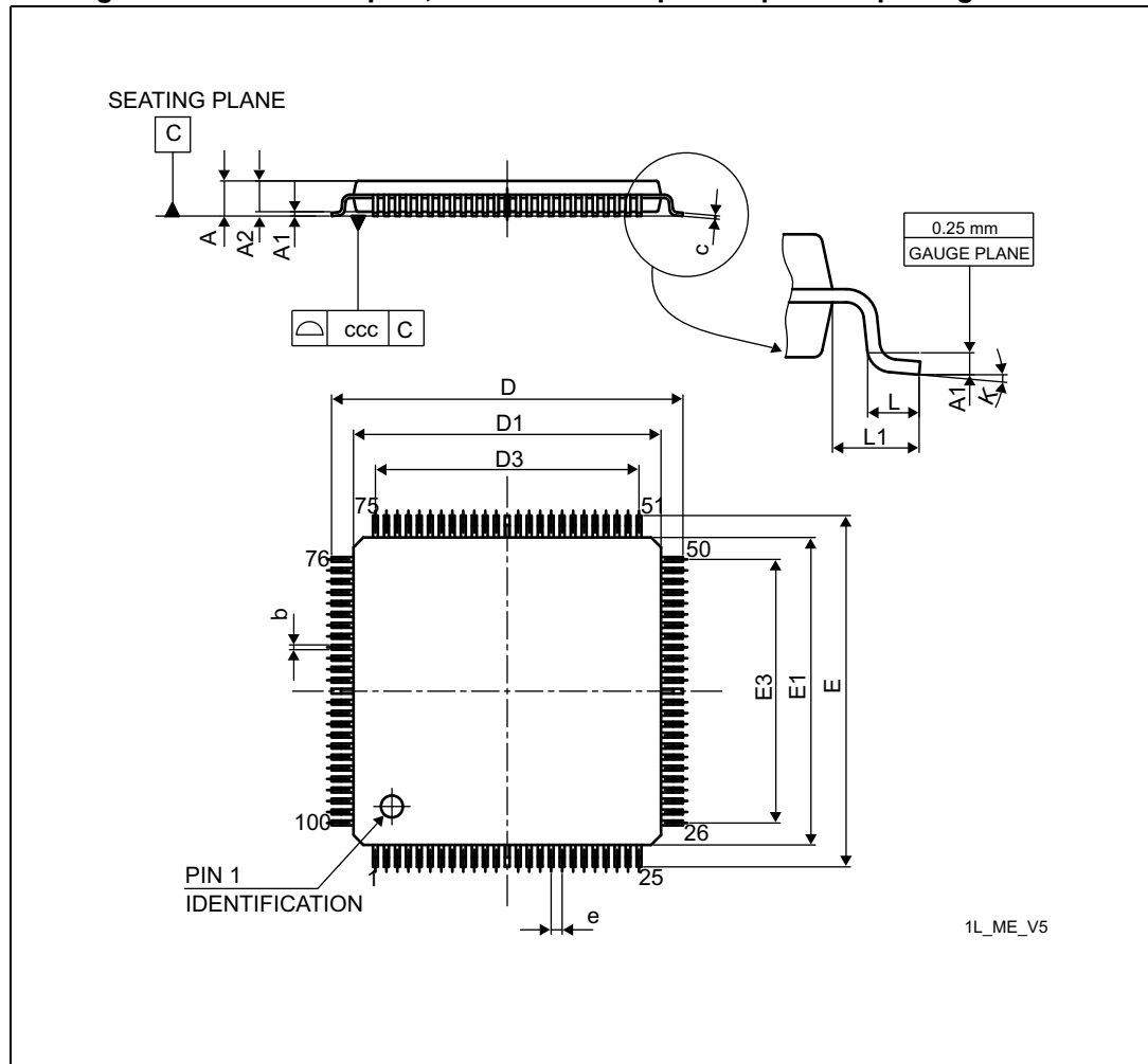
Figure 42. LQFP - 100 pins, 14 x 14 mm low-profile quad flat package outline
