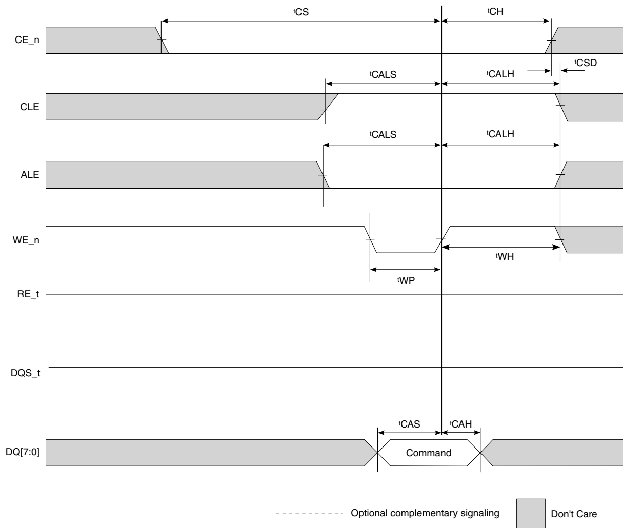
Figure 68. Command cycle
