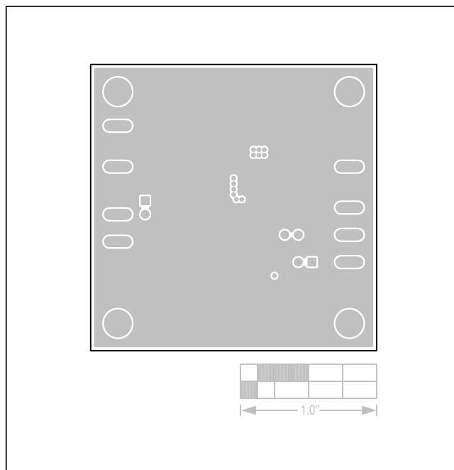
Figure 14. MAX17544 5V Output EV Kit PCB Layout—Inner Layer 1
