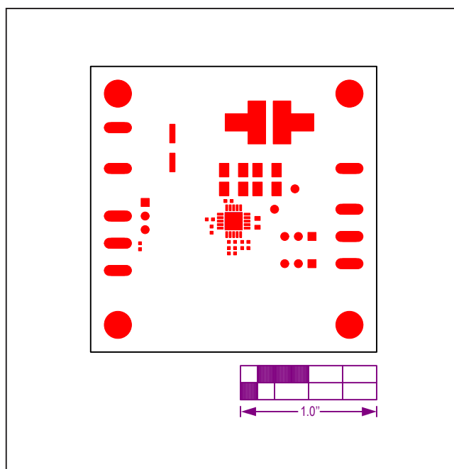
Figure 17. MAX17544 5V Output EV Kit Component Placement Guide—Top Solder Mask
