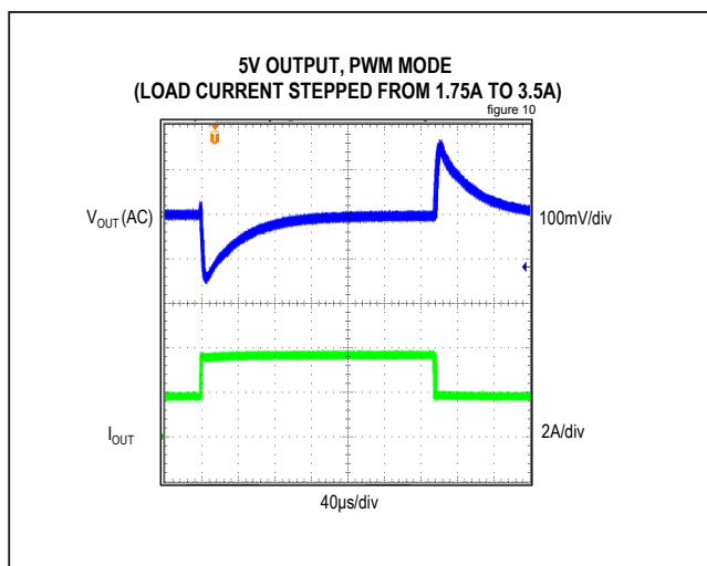
Figure 10. MAX17544 5V Output, 1.75A to 3.5A Load Transient
