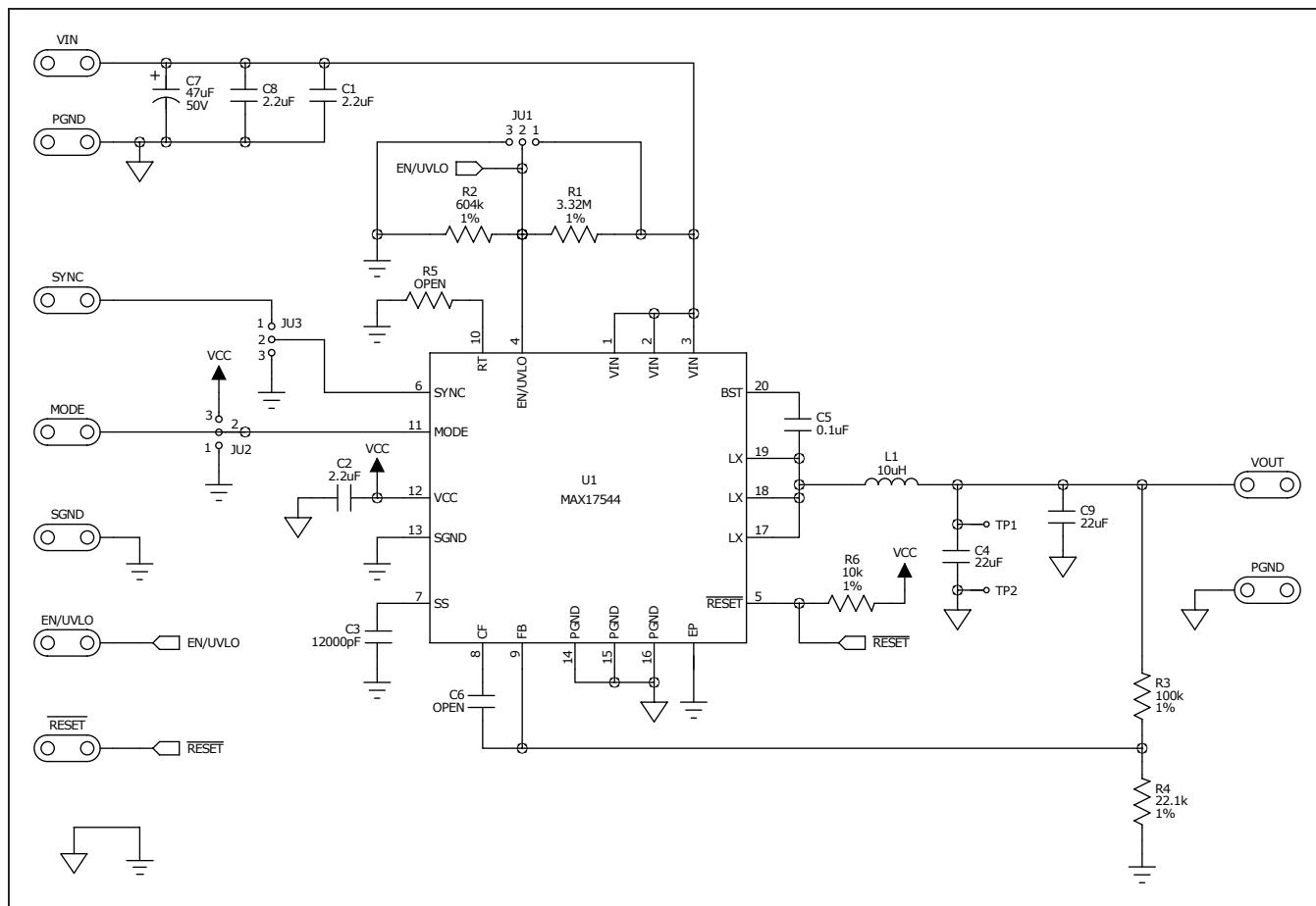
Figure 11. MAX17544 5V Output EV Kit Schematic
