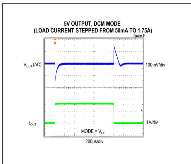
Figure 9. MAX17544 5V Output, 50mA to 1.75A Load Transient (DCM Mode)
