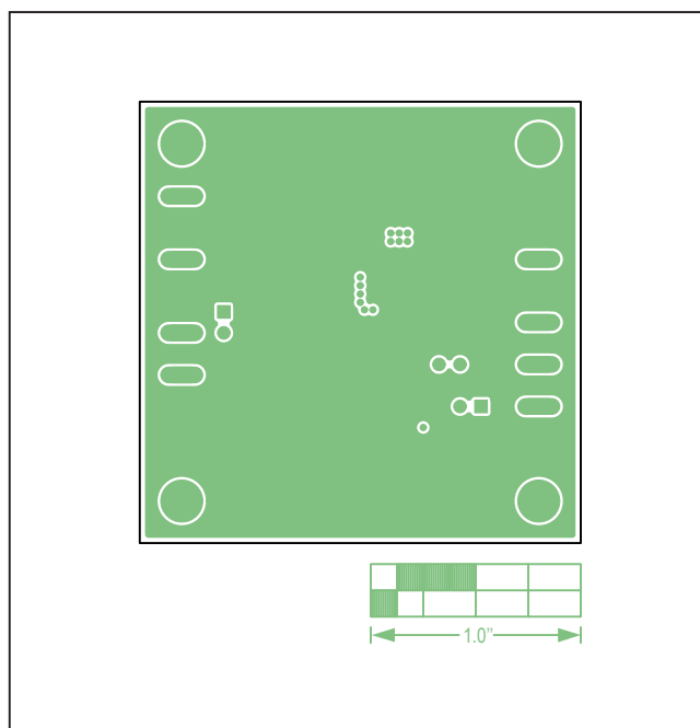
Figure 15. MAX17544 5V Output EV Kit PCB Layout—Inner Layer 2
