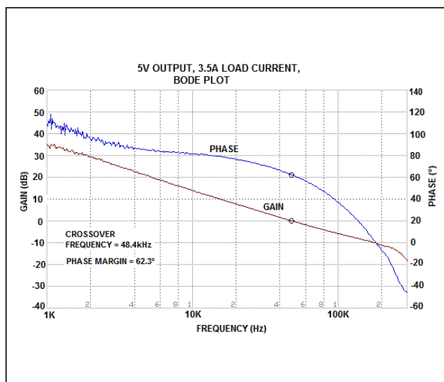
Figure 6. MAX17544 5V Output Full Load Bode Plot ( V_{IN} = 24V )
