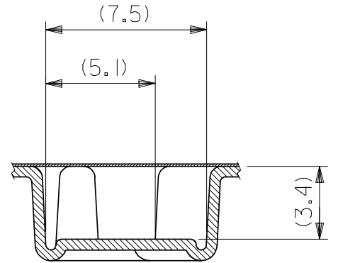
SECT:X-X (SCALE 4:1)
