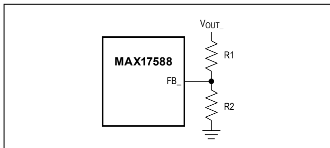
Figure 4. Output-Voltage Programming
