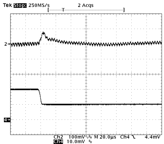
Fig-2.0V-7: Output voltage response for V_{out}=2.0V to negative load current step change from 10A to 5A with slew rate of -5A/us at V_{in}=12V . C_o=47\mu F \times 2 ceramic. Top trace: output voltage (100mV/div.) Bottom trace: load current (5A/div.) Time scale: 20us/div.
