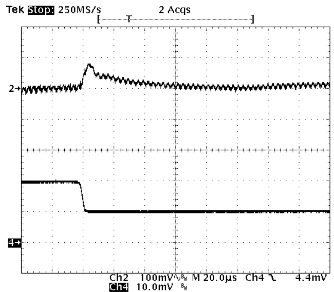
Fig-1.5V-7: Output voltage response for V_{out}=1.5V to negative load current step change from 10A to 5A with slew rate of -5A/us at V_{in}=12V . C_o=47\mu F \times 2 ceramic. Top trace: output voltage (100mV/div.) Bottom trace: load current (5A/div.) Time scale: 20us/div.
