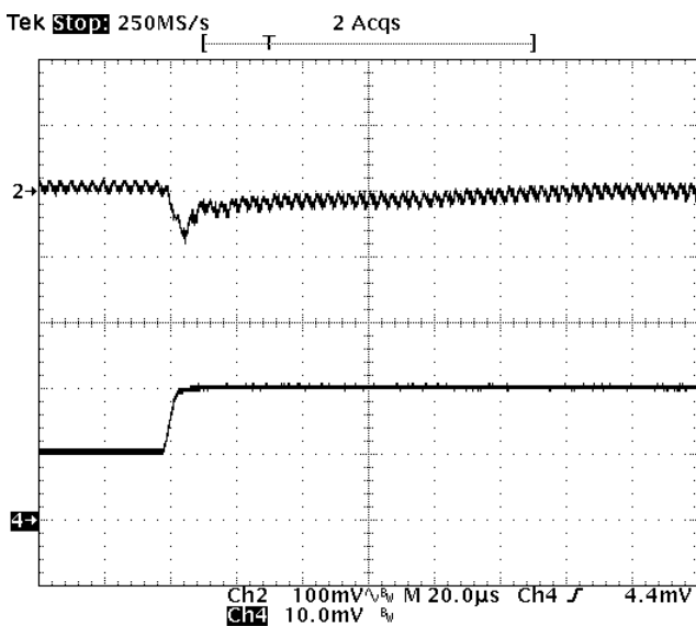
Fig-2.0V-6: Output voltage response for V_{out}=2.0V to positive load current step change from 5A to 10A with slew rate of 5A/us at V_{in}=12V . C_o=47\mu F \times 2 ceramic. Top trace: output voltage (100mV/div.) Bottom trace: load current (5A/div.) Time scale: 20us/div.
