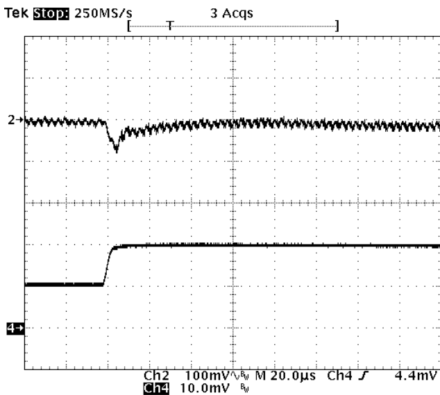
Fig-1.5V-6: Output voltage response for V_{out}=1.5V to positive load current step change from 5A to 10A with slew rate of 5A/us at V_{in}=12V . C_o=47\mu F \times 2 ceramic. Top trace: output voltage (100mV/div.) Bottom trace: load current (5A/div.) Time scale: 20us/div.
