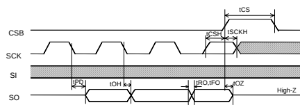
Figure 2. Input / Output timing
