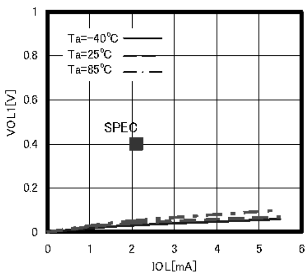
Figure 6. "L" Output Voltage V_{OL1}(V_{CC}=2.5\text{V})
