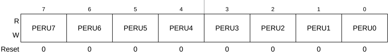
Figure 2-82. Port U Pull Device Enable Register (PERU)
