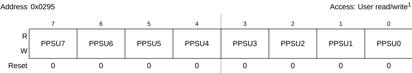
Figure 2-83. Port U Polarity Select Register (PPSU)
