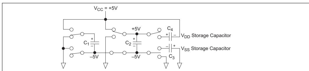
Figure 17. Charge Pump — Phase 3
