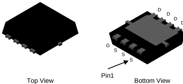
PowerDI3333-8 (SWP) (Type UX)
