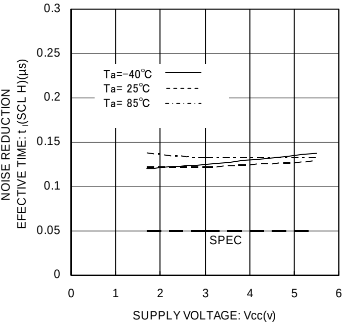
Figure 28. Noise Spike Width t_l (SCL H)
