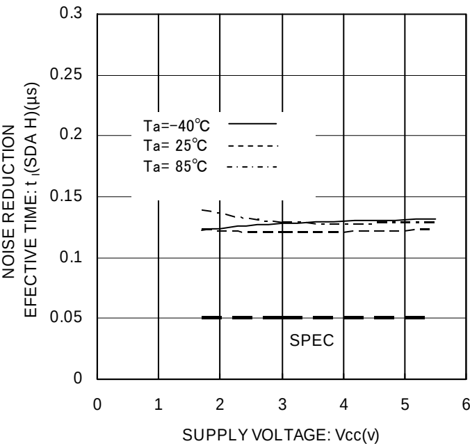
Figure 30. Noise Spike Width t_l (SDA H)
