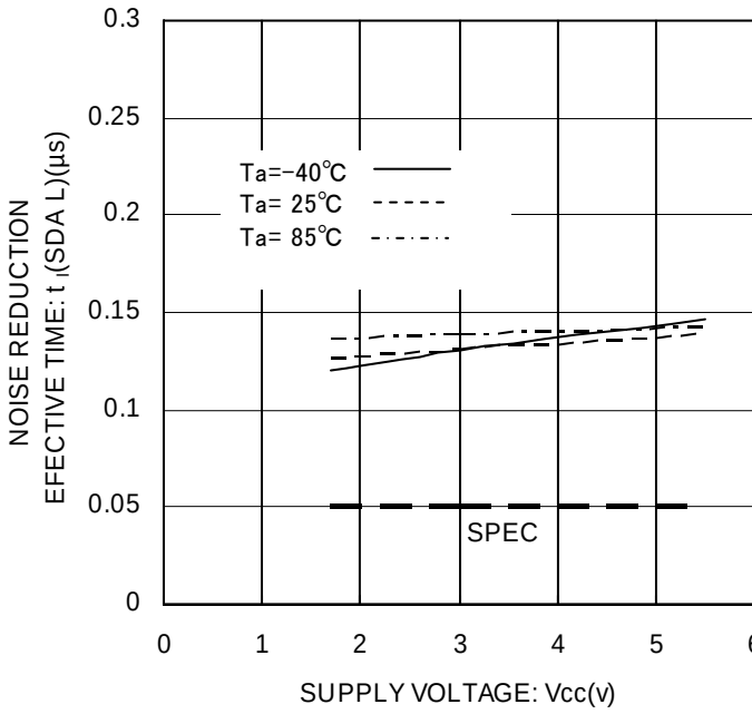
Figure 31. Noise Spike Width t_l (SDA L)
