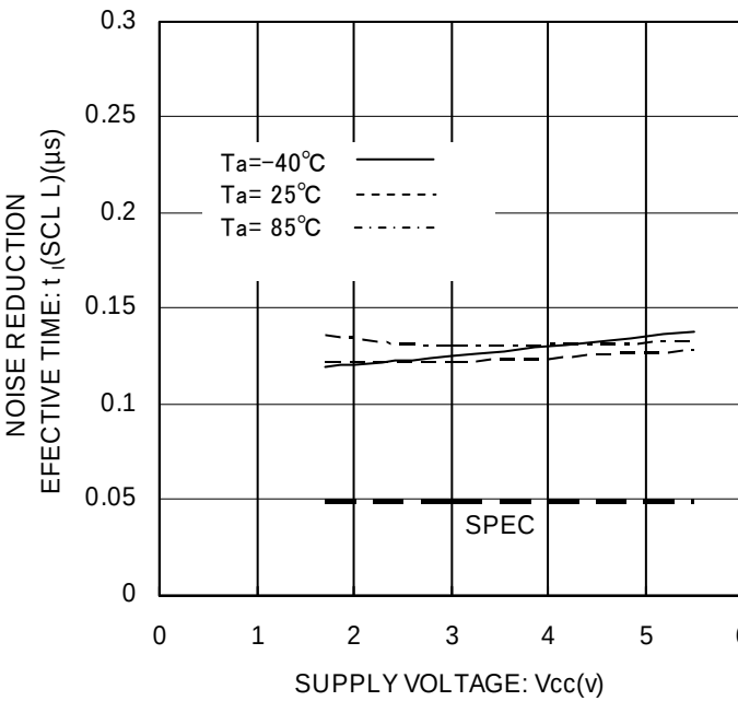
Figure 29. Noise Spike Width t_l (SCL L)
