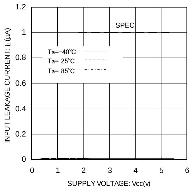
Figure 8. Input Leakage Current I_L (A1, A2, SCL, WP)
