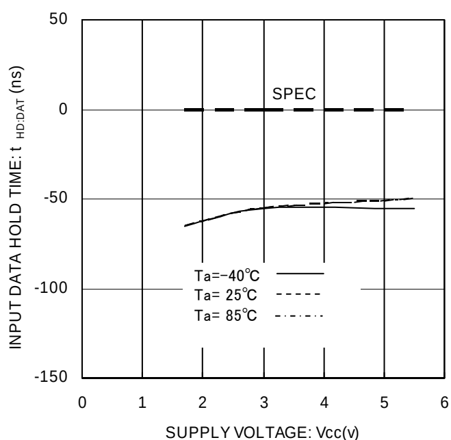
Figure 19. Input Data Hold Time t_{HD:DAT}(\text{HIGH})
