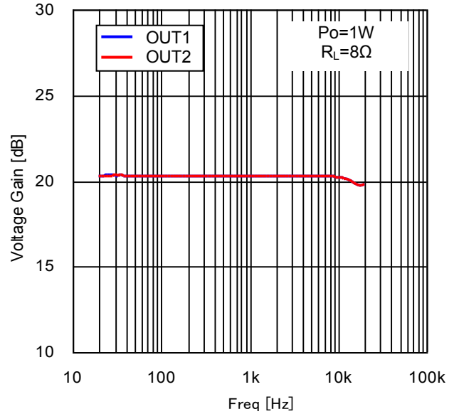
Figure 22. Voltage Gain vs Freq (8Ω)
