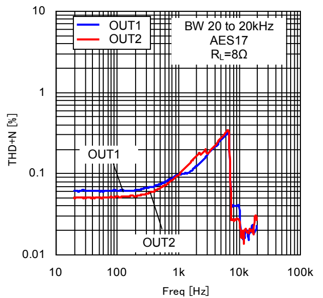
Figure 24. THD+N vs Freq (8Ω)
