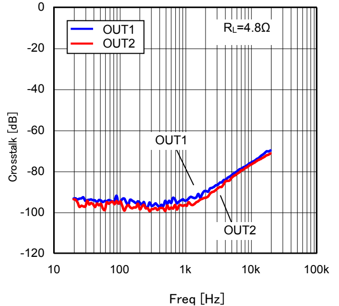
Figure 44. Crosstalk vs Freq (4.8 \Omega )
