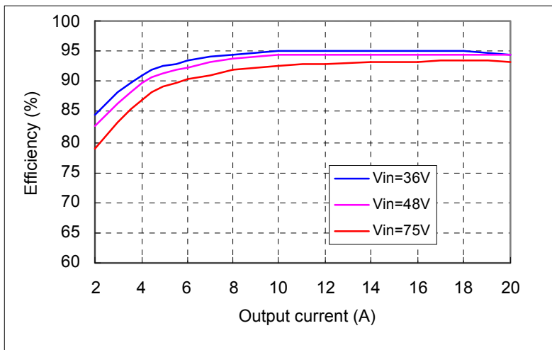
Figure 1 Efficiency vs. output current, T_a=25^{\circ}\text{C} , T_c=40^{\circ}\text{C} , V_o=30\text{V}
