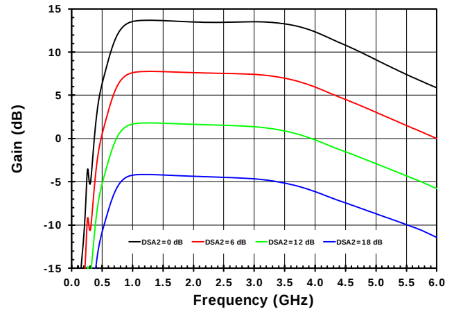
Figure 5. Gain vs. Frequency for DSA2 Settings
