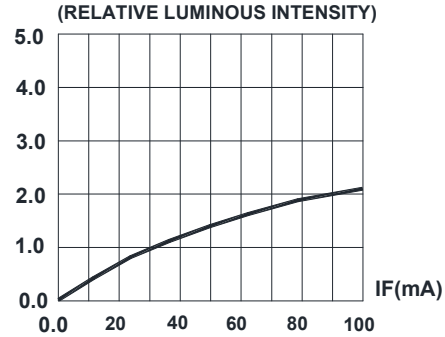
FIG.2 RELATIVE LUMINOUS INTENSITY VS. FORWARD CURRENT (RELATIVE LUMINOUS INTENSITY)
