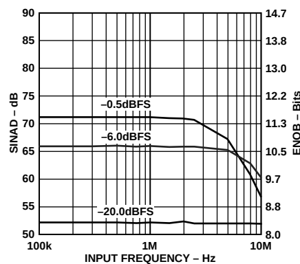
Figure 14. SINAD vs. Input Frequency (Input Span = 2 V, V_{CM} = 2.5\text{ V} )
