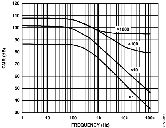
Figure 17. CMR vs. Frequency, = 5 V_S, 0 V_S, V_{REF} = 2.5 V
