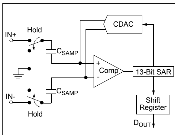
FIGURE 5-1: Simplified Block Diagram.
