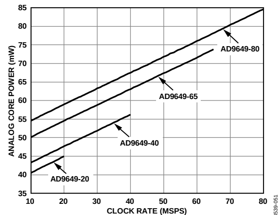
Figure 54. Analog Core Power vs. Clock Rate
