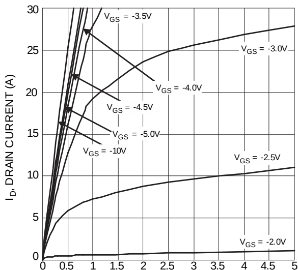
Figure 12 Typical Output Characteristics
