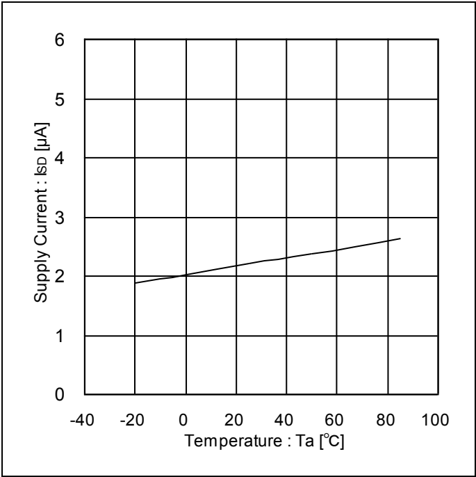
Figure 4. Supply Current vs Temperature ("Power-down Current", V CC =3.0V)
