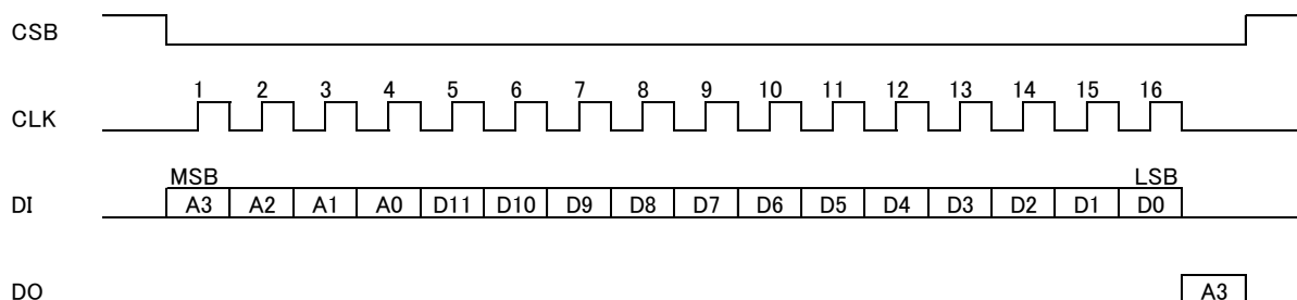
Figure 12. Communication Format
