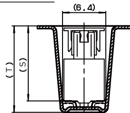
SECT. F-F
