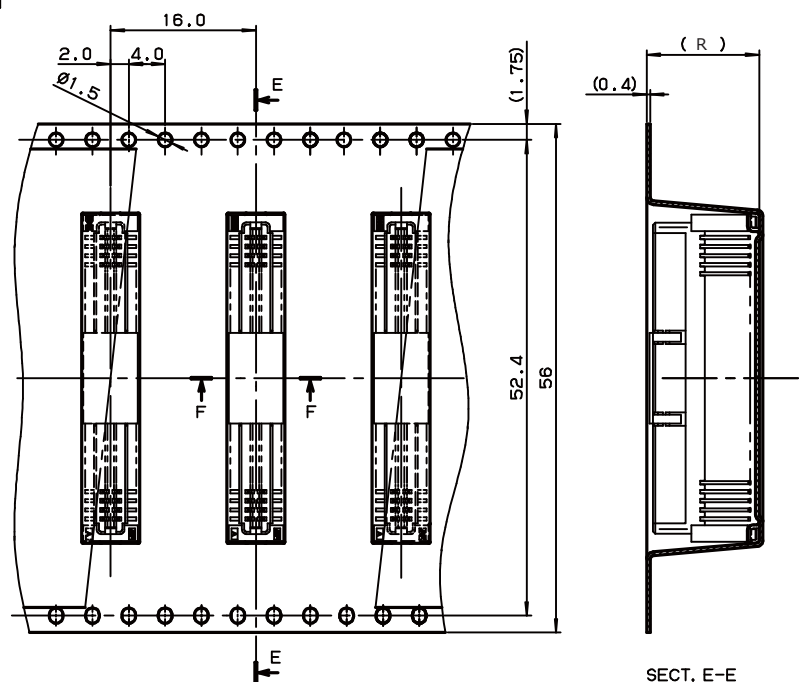
SECT. E-E
