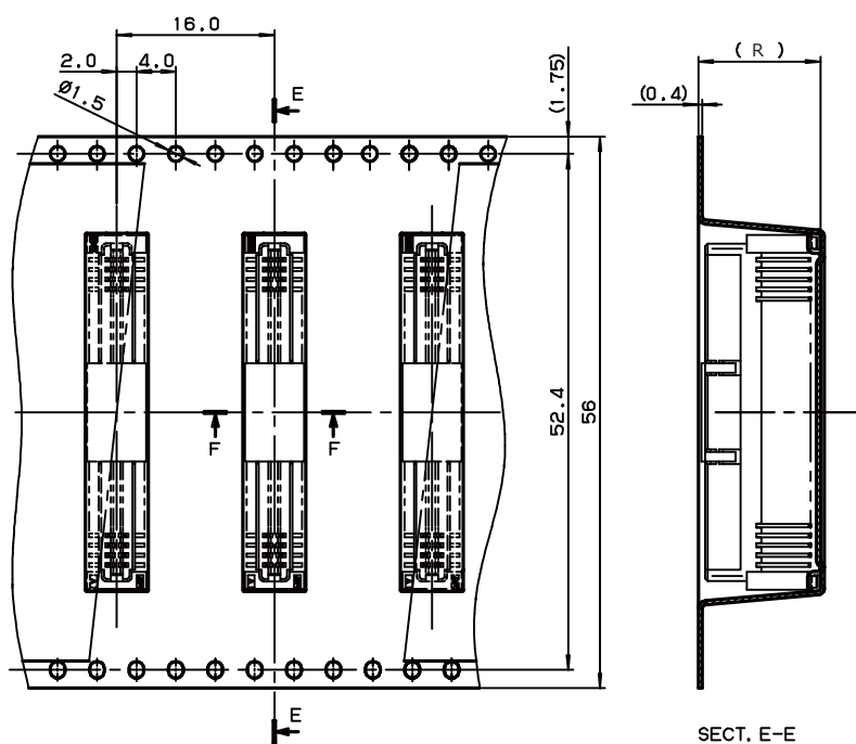
SECT. E-E
