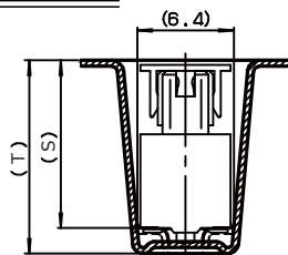
SECT. F-F
