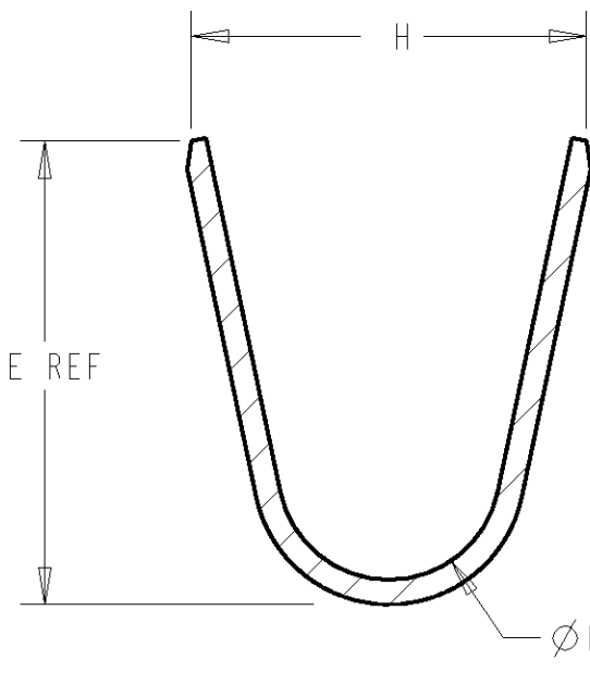
SECTION G-G
