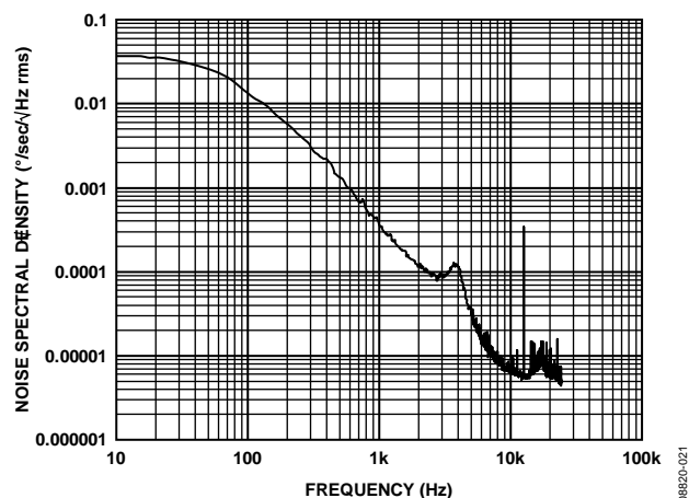
Figure 22. Noise Spectral Density with Additional 250 Hz Filter
