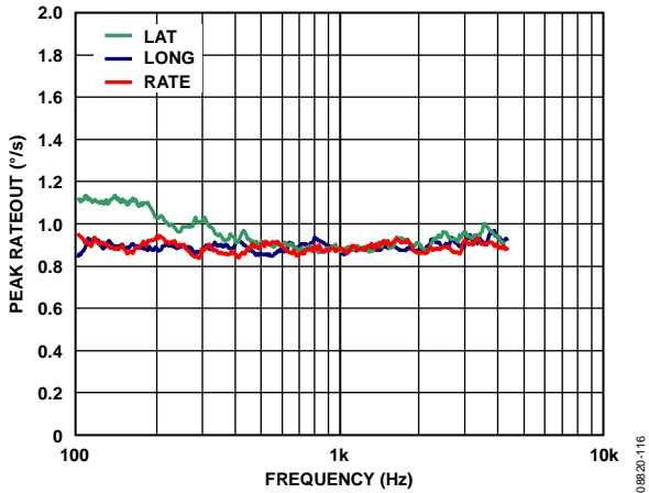
Figure 16. Typical Response to 10 g Sinusoidal Vibration (Sensor Bandwidth = 40 Hz)
