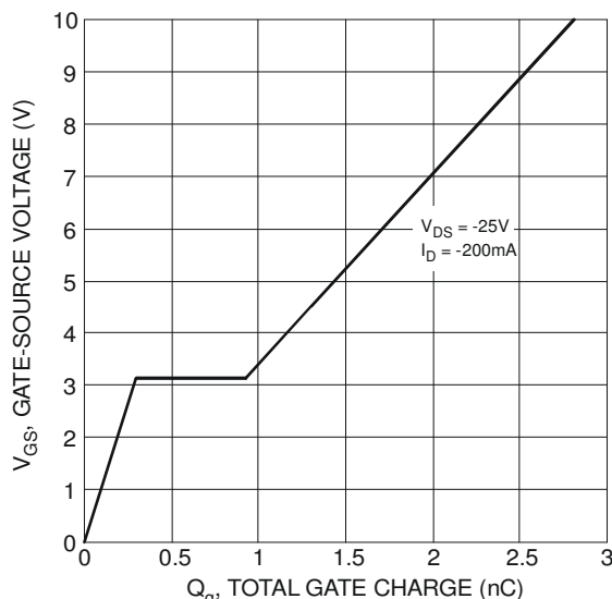
Figure 10 Gate-Charge Characteristics
