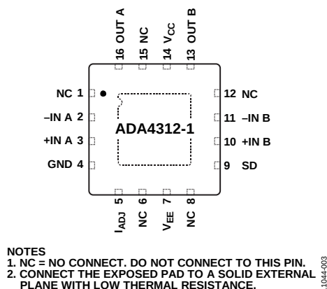
Figure 3. Pin Configuration
