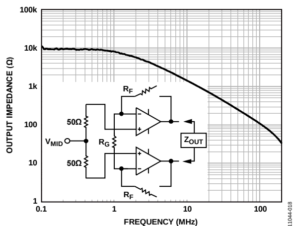
Figure 10. Open-Loop Disabled Differential Output Impedance vs. Frequency
