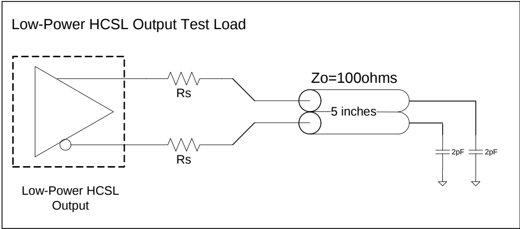
Alternate Differential Output Terminations
