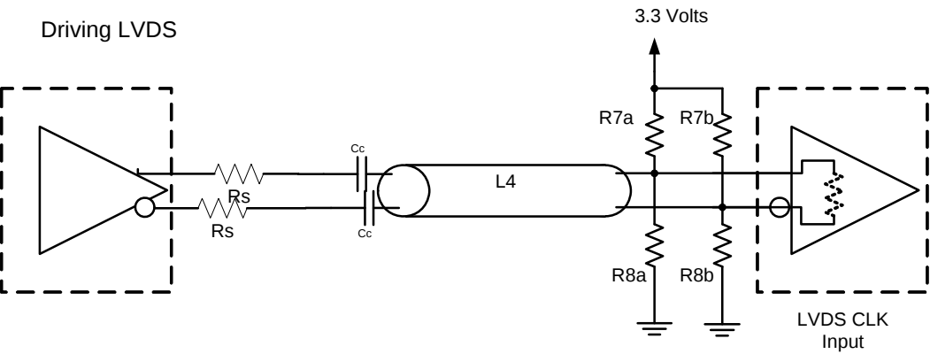
Driving LVDS inputs
