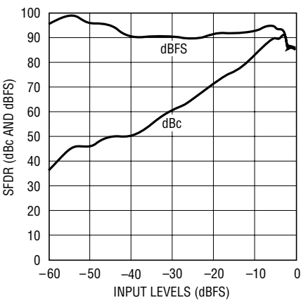
LTC2221: SFDR vs Input Level, f_{IN} = 70\text{MHz} , 2V Range
