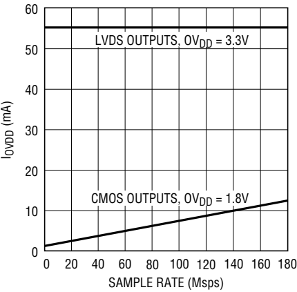
LTC2221: I_{OVDD} vs Sample Rate, 5MHz Sine Wave Input, -1\text{dB}
