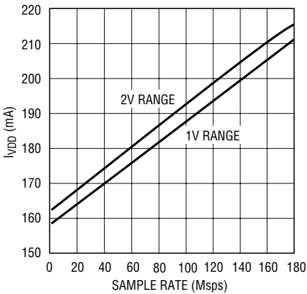
LTC2221: I_{VDD} vs Sample Rate, 5MHz Sine Wave Input, -1\text{dB}
