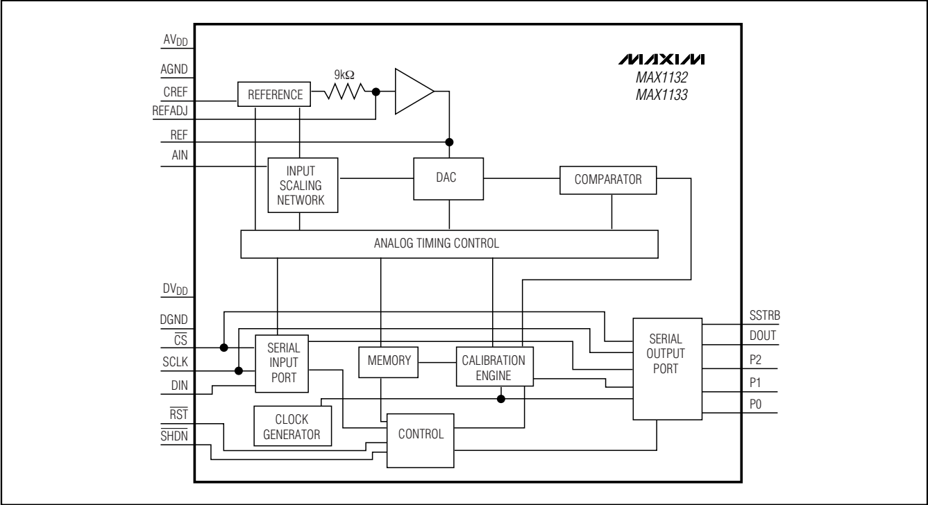
Functional Diagram
