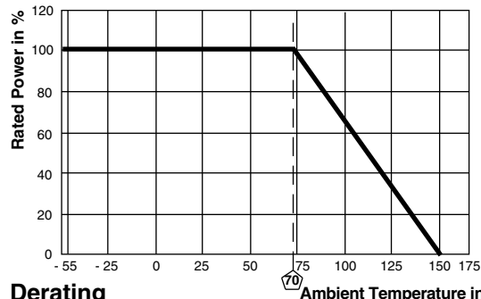
Derating
