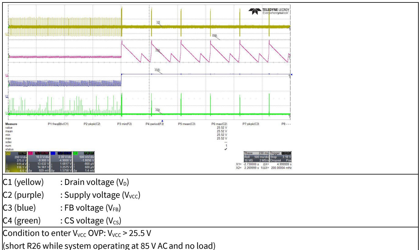
Figure 29 V_{CC} OVP
