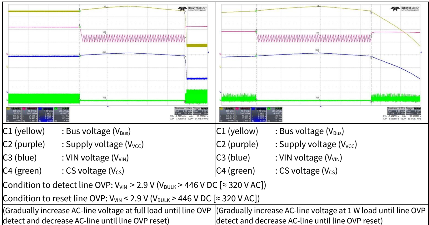
Figure 28 Line OVP
