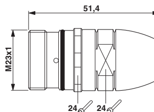
Dimensional drawing
