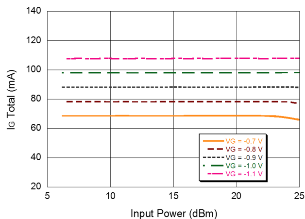
Gate Current vs. Input Power @ 9 GHz
