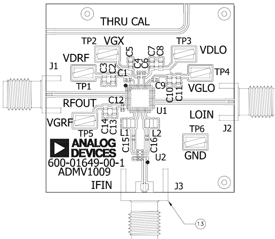
Figure 62. ADMV1009-EVALZ Evaluation Board Top Layer
