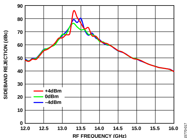
Figure 17. Sideband Rejection vs. RF Frequency at Various LO Powers
