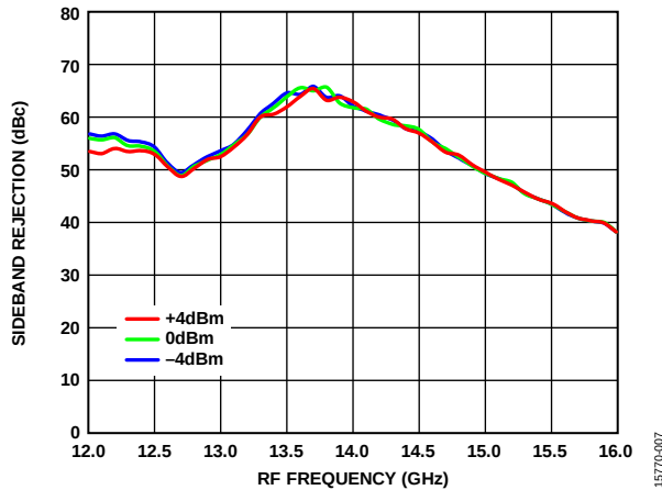
Figure 7. Sideband Rejection vs. RF Frequency at Various LO Powers
