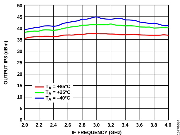
Figure 34. Output IP3 vs. IF Frequency at Various Temperatures
