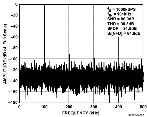
Figure 7. FFT Plot
