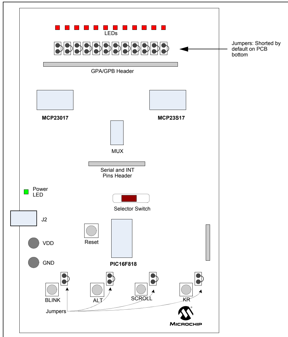
FIGURE 2-1: BOARD LAYOUT
