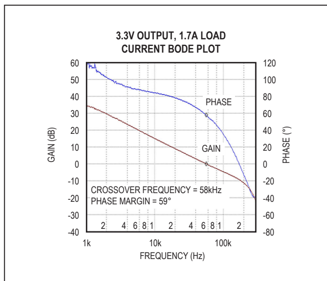
Figure 6. MAX17545 3.3V Output Full Load Bode Plot ( V_{IN} = 24V )
