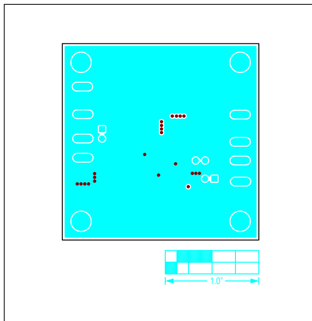
Figure 14. MAX17545 3.3V Output EV Kit PCB Layout—Inner Layer 1
