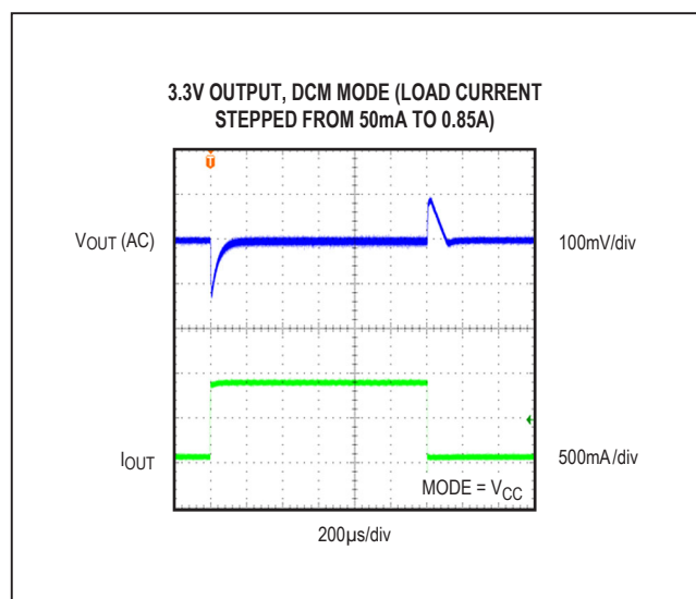
Figure 9. MAX17545 3.3V Output, 50mA to 0.85A Load Transient (DCM Mode)
