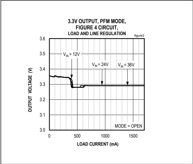
Figure 3. MAX17545 3.3V Output Load and Line Regulation (PFM Mode)
