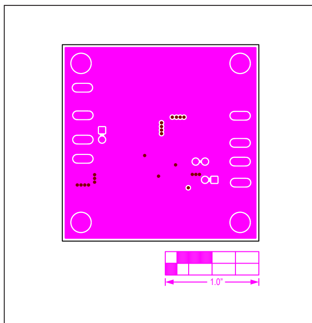
Figure 15. MAX17545 3.3V Output EV Kit PCB Layout—Inner Layer 2
