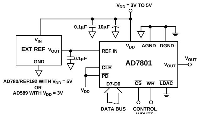
Figure 28. Typical Configuration Using An External Reference
