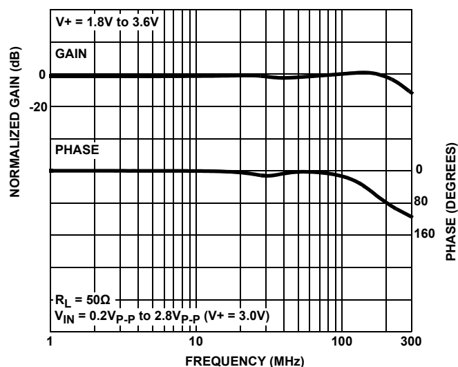
FIGURE 14. FREQUENCY RESPONSE
