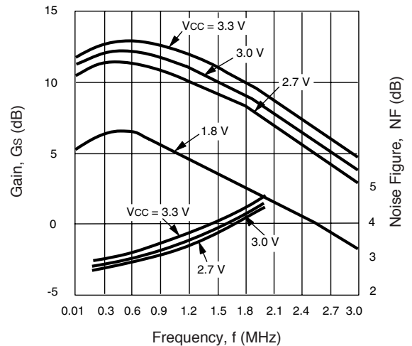
UPC2747TB GAIN AND NOISE FIGURE vs. FREQUENCY
