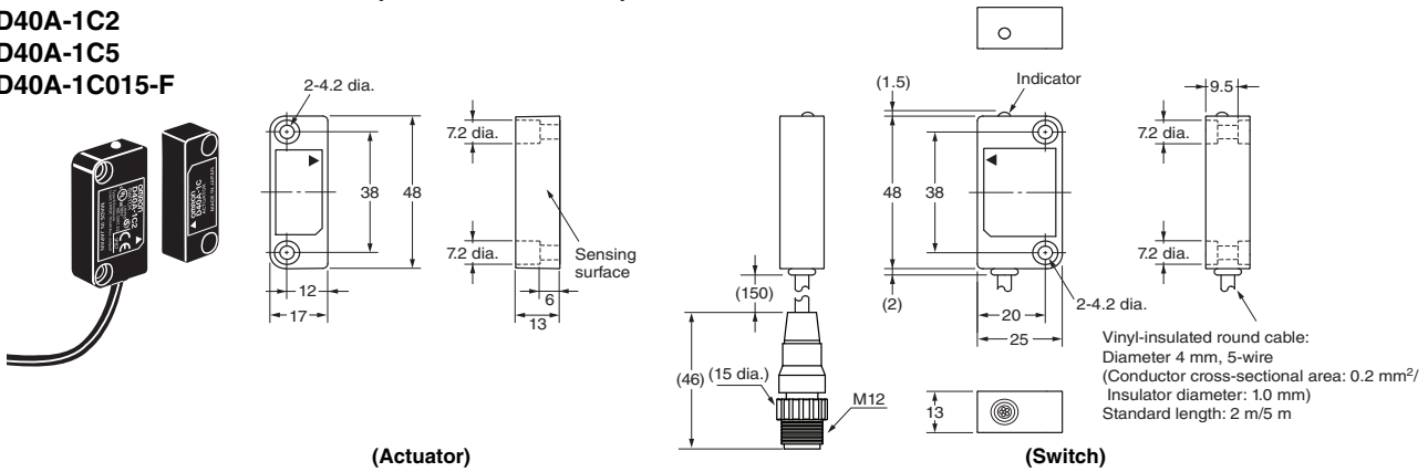
(Actuator)
