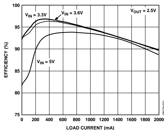
Figure 2. Efficiency vs. Load Current for the ADP2107 with V_{OUT} = 2.5\text{ V}
