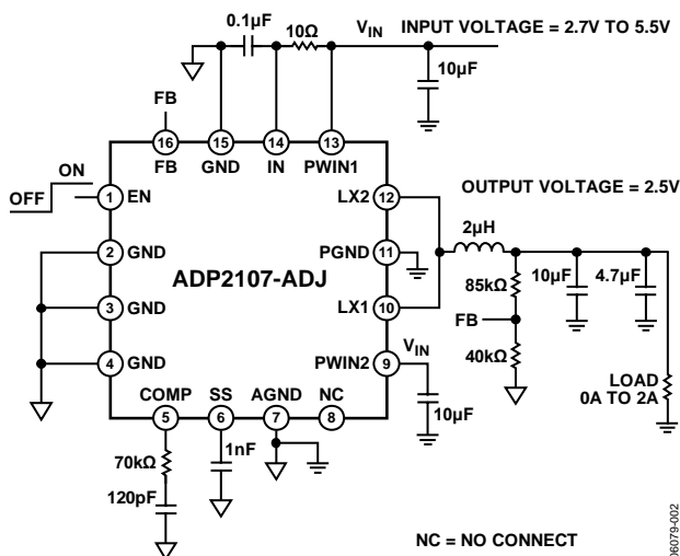
Figure 1. Circuit Configuration of ADP2107 with V_{OUT} = 2.5\text{ V}
